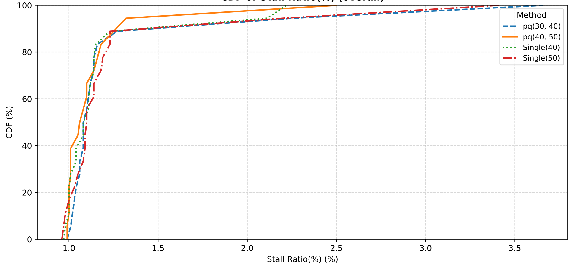
CDF of Stall Ratio(%) (overall)
